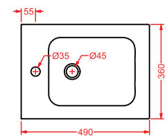
BKB002 BLOCK bidet terra back to wall bidet
